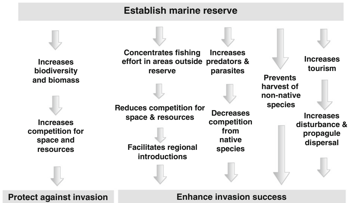
Fig. 1 Theoretical pathways by which marine reserves resist or enhance non-native species
